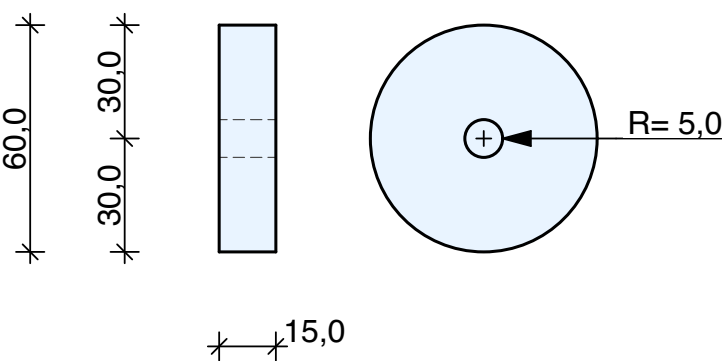
Pos_8.5 4 Pieces
