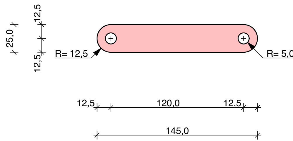
Pos_6.3.3 2 Pieces Sheet Metal 5 mm
