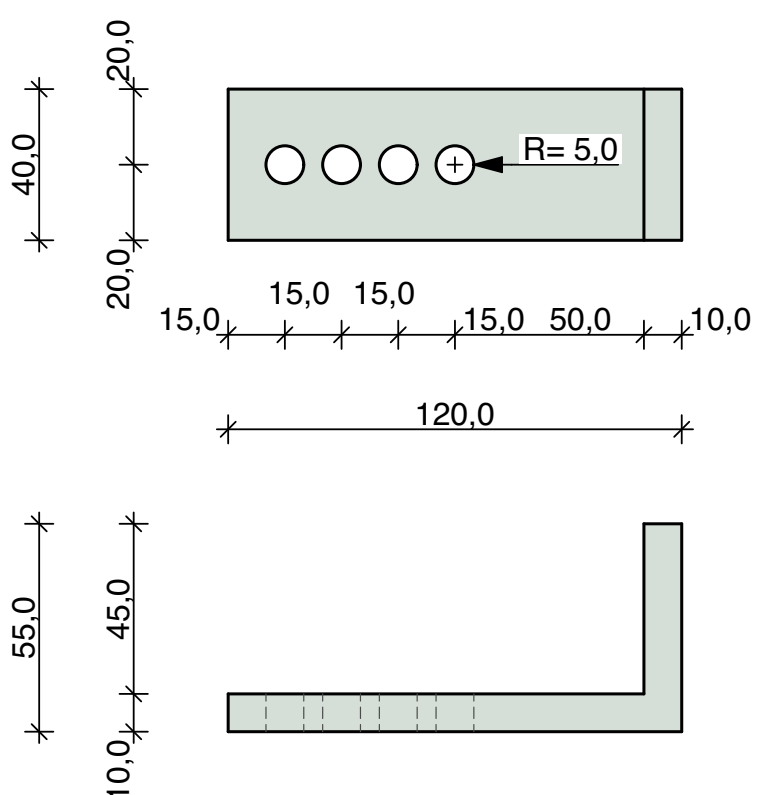
Pos_3.13 2 Pieces Sheet Metal 10 mm, welded
