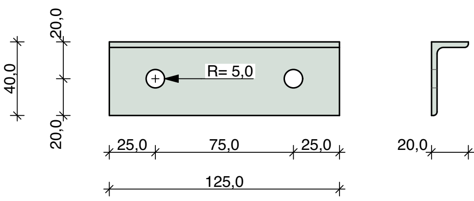
Pos_3.16 2 Pieces L-Section 40 x 20 x 3 mm
