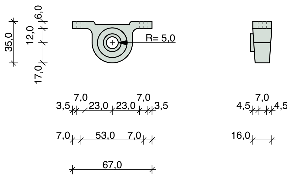
Pos_3.4 2 Pieces Pillow Block Bearing 10 mm Inner Diameter
