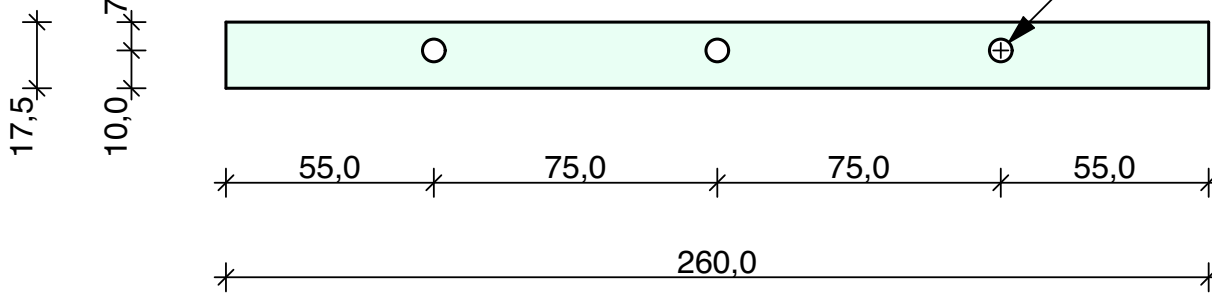
Pos_5.4 2 Pieces Hard Plastic 5 mm
