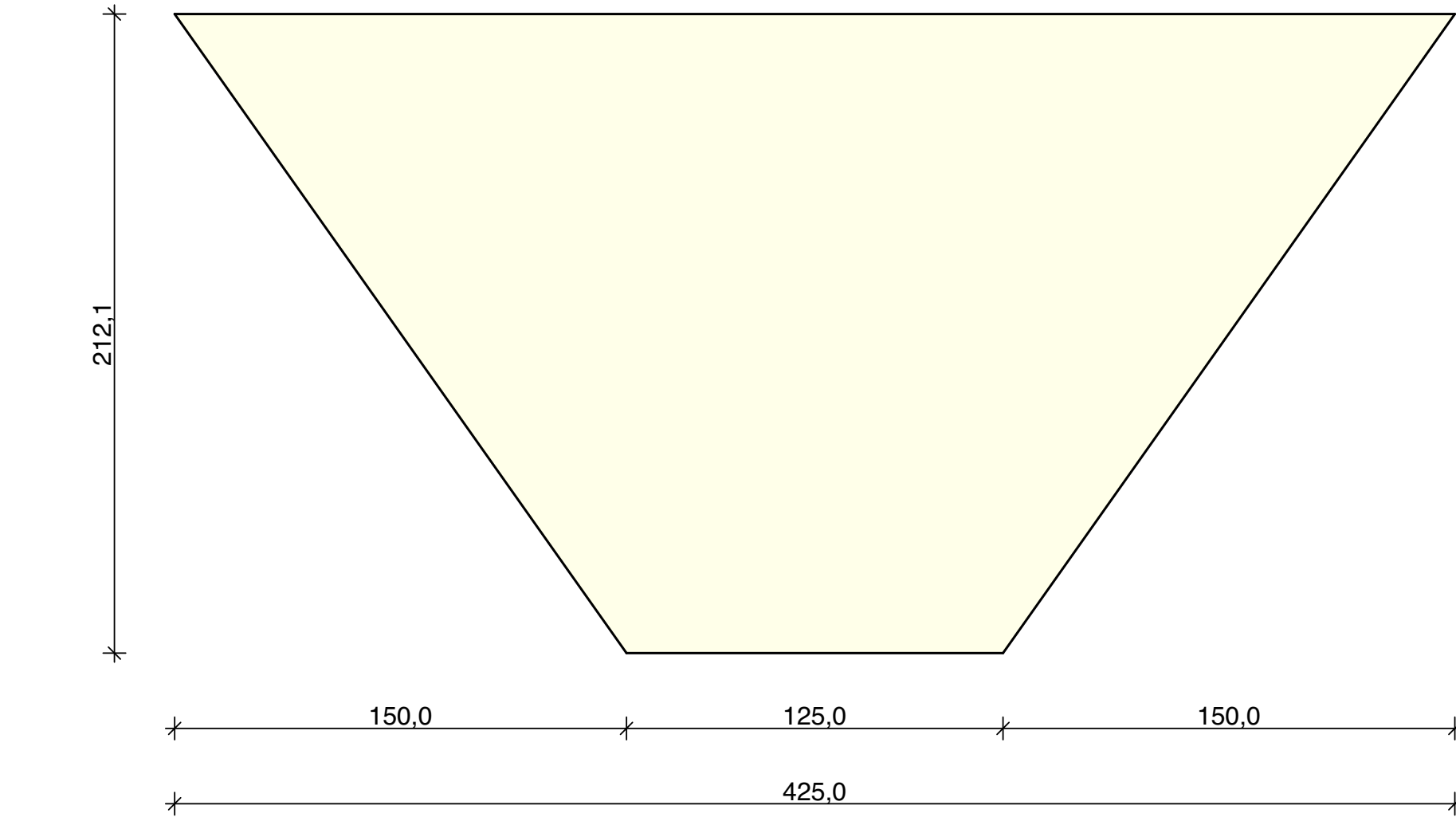
Pos_9.6 1 Piece Sheet Metal 3 mm
