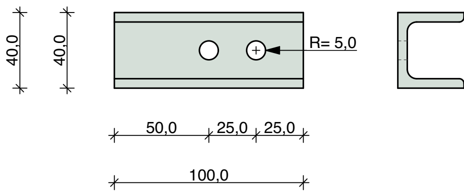
Pos_3.9 1 Piece UPN 40 x 35 mm
