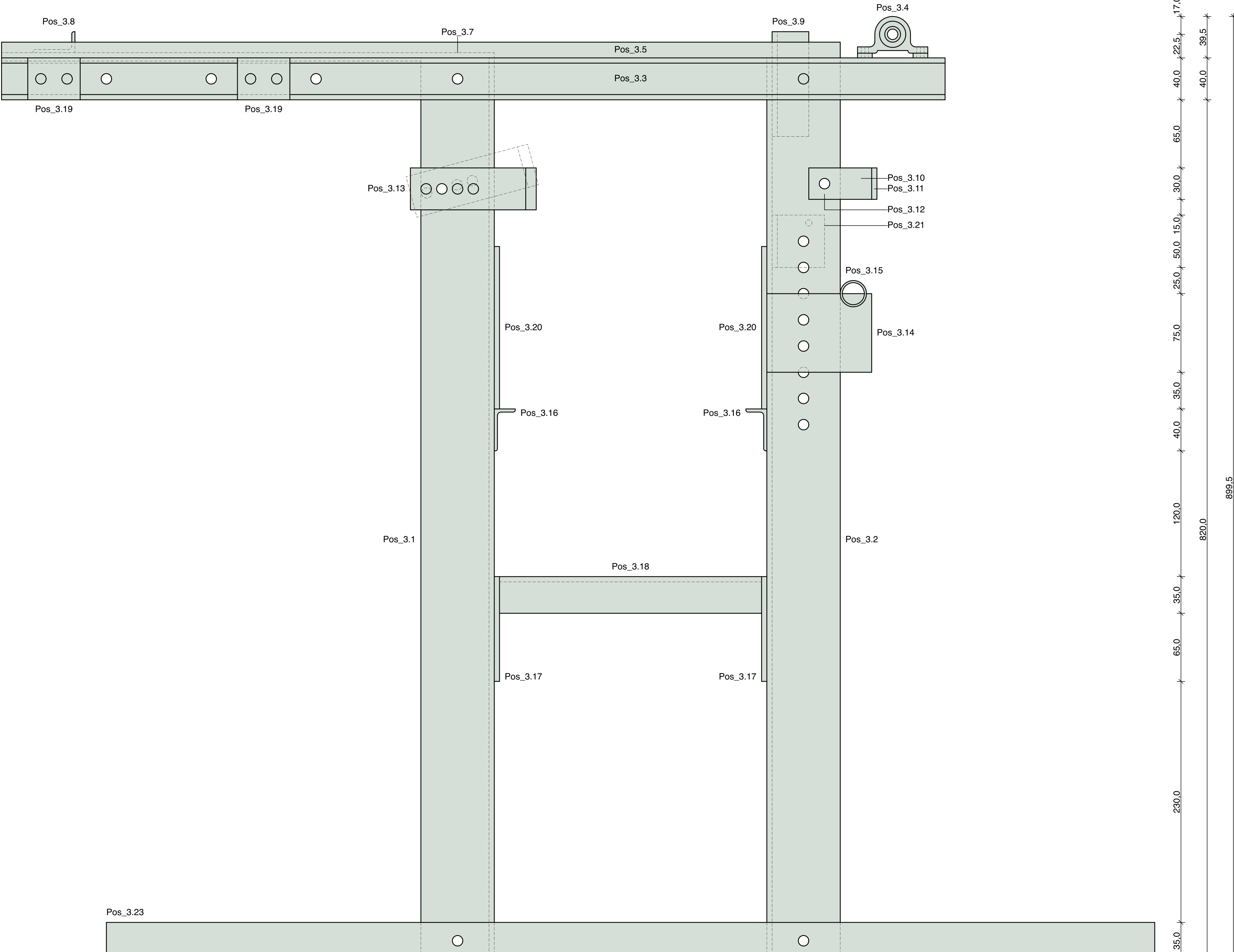
Assembly Side View
