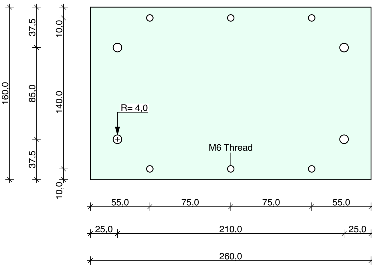
Pos_5.1 1 Piece Sheet Metal 5 mm
