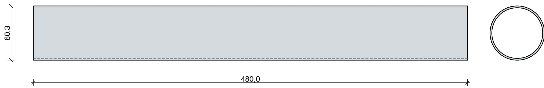
Pos_7.1 2 Pieces Circular Hollow Section 60,3 x 2 mm
