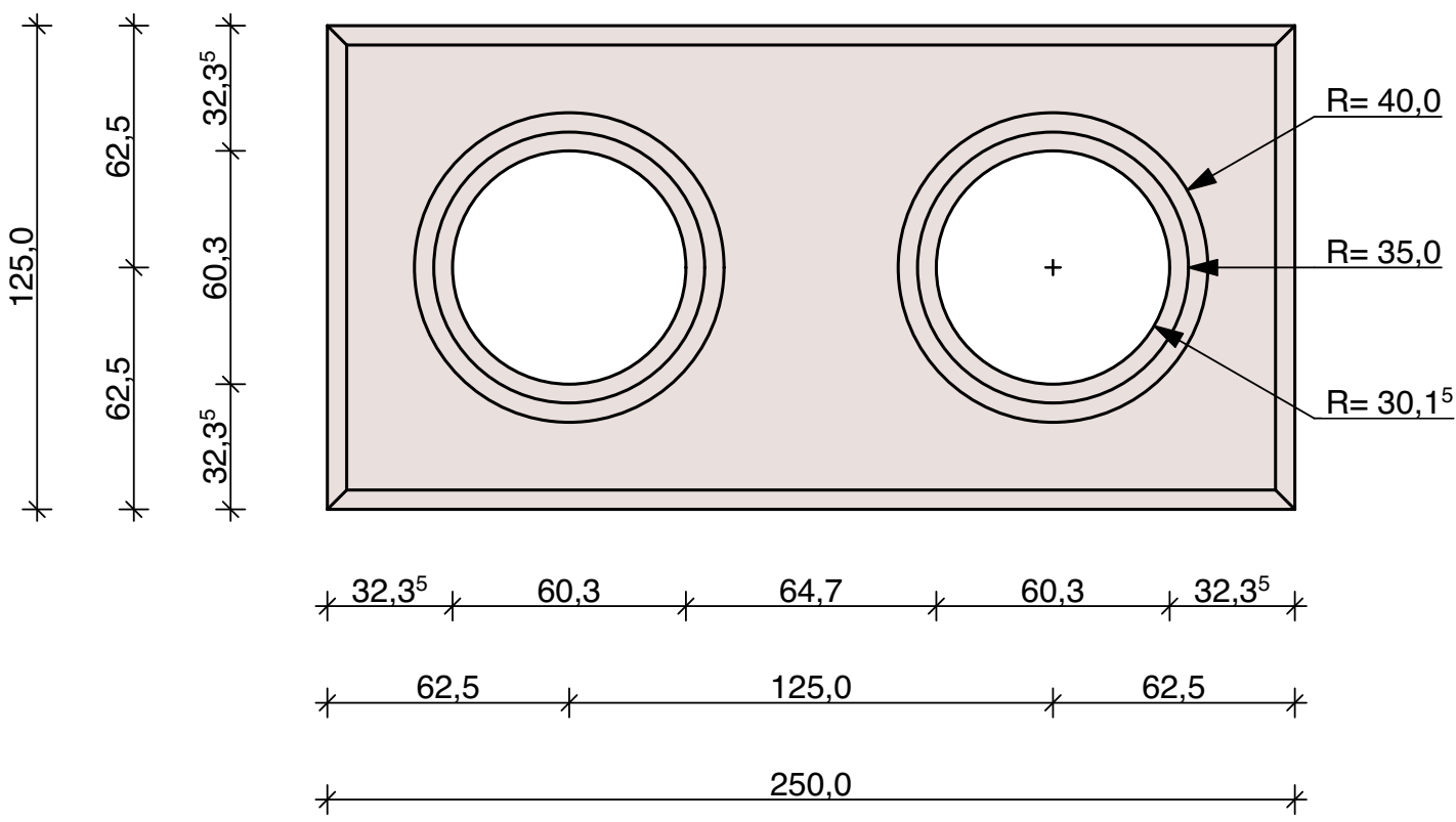
Top View
