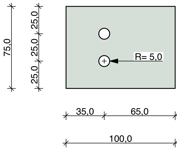
Pos_3.14 2 Pieces Sheet Metal 5 mm
