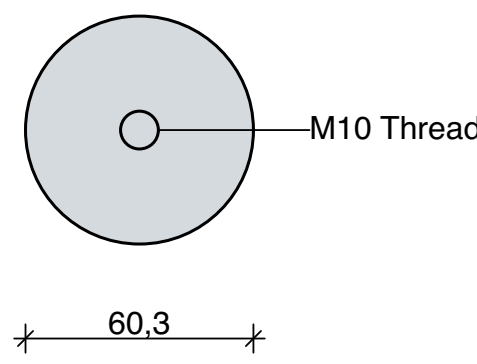
Pos_7.3 2 Pieces Sheet Metal 10 mm
