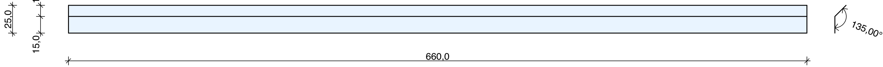
Pos_8.6 2 Pieces
