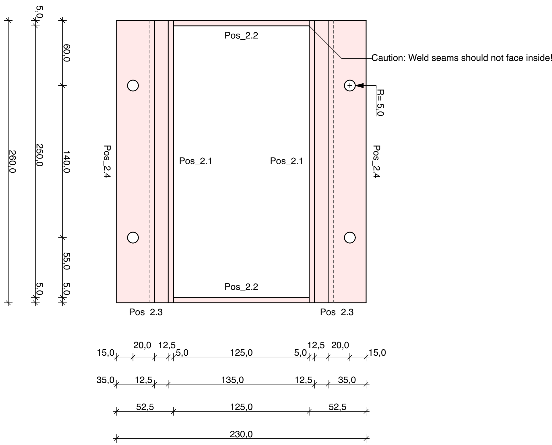
Assembly_Section
