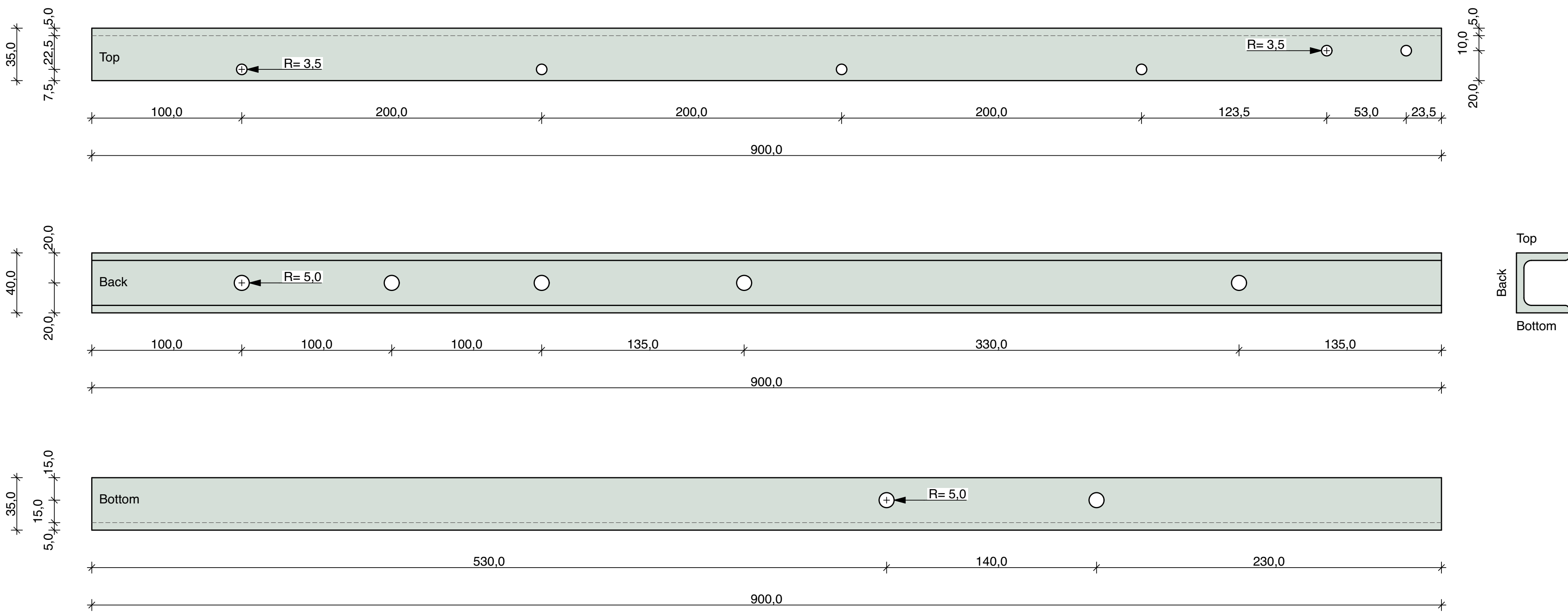
Pos_3.3 2 Pieces (Pieces are mirrored!) UPN 40 x 35 mm
