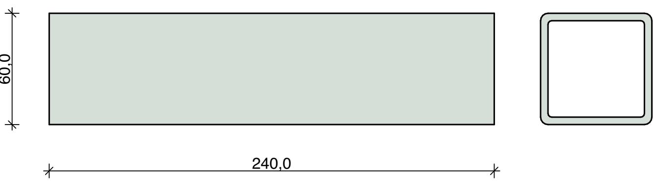
Pos_6.2.2 1 Piece Square Hollow Section 60 x 60 x 4 mm
