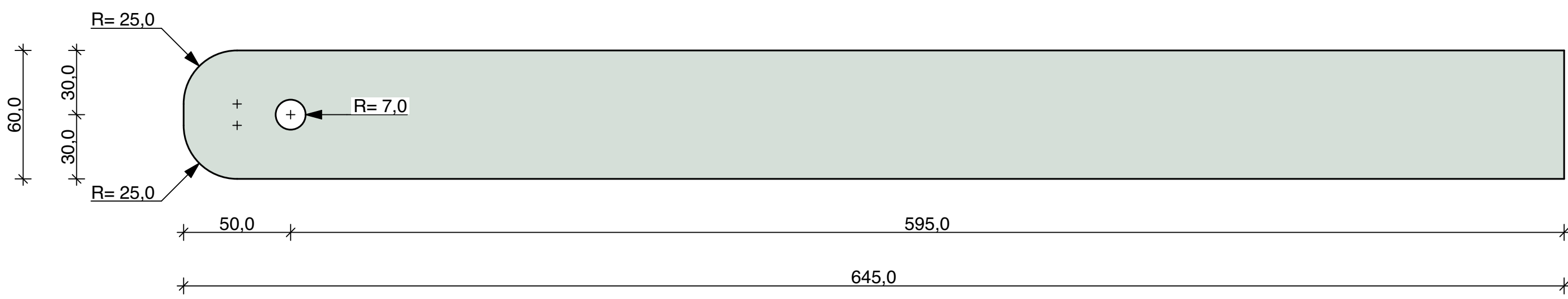
Pos_6.2.1 2 Pieces Sheet Metal 10 mm
