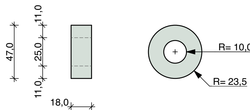
Pos_6.2.6 1 Piece Bearing 20 x 47 x 18 mm
