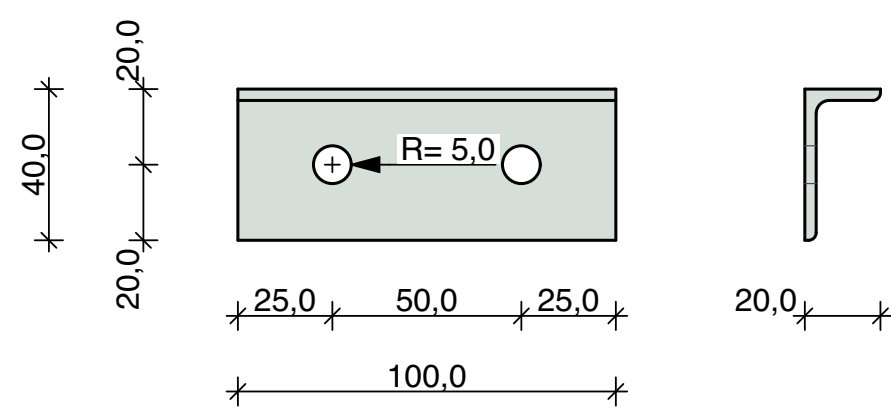
Pos_3.8 1 Piece L-Section 40 x 20 x 3 mm
