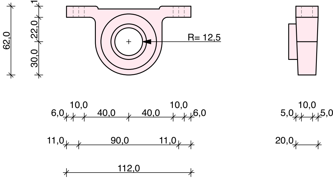
Pos_4.10 2 Pieces Pillow Block Bearing 25 mm Inner Diameter
