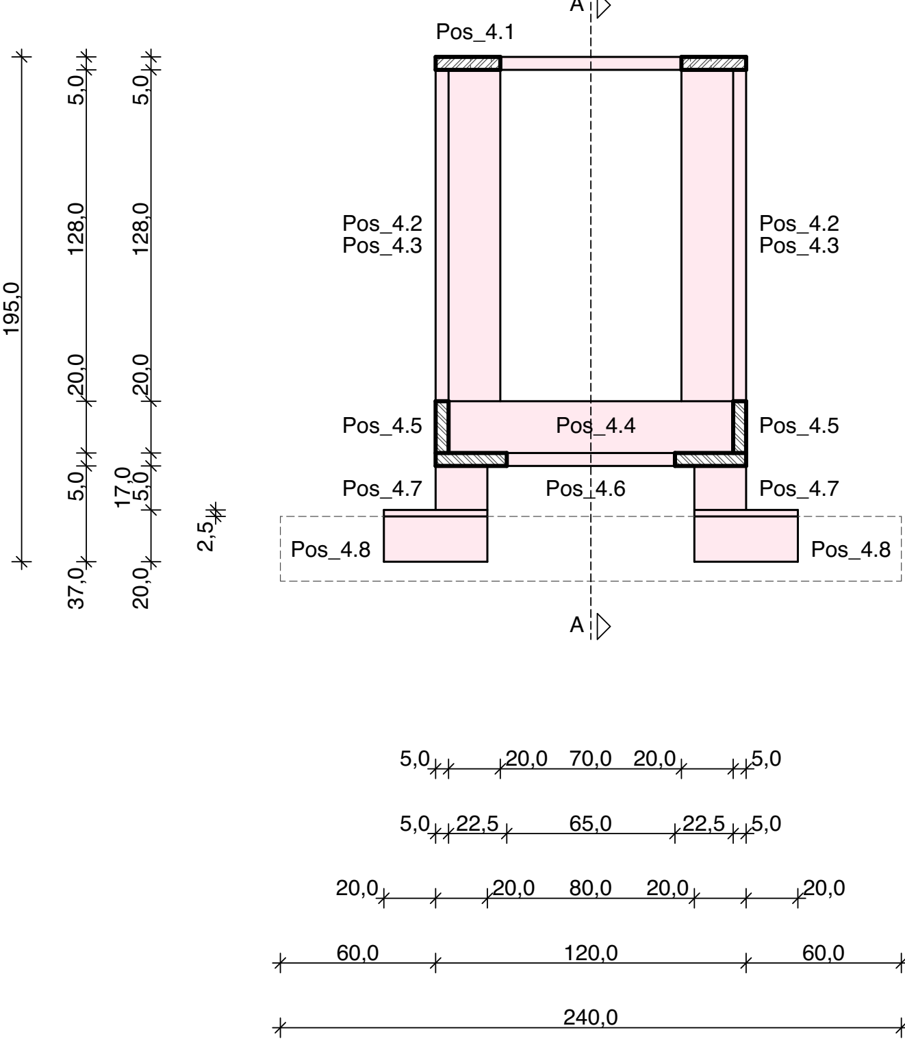
Assembly_Section (C-C)
