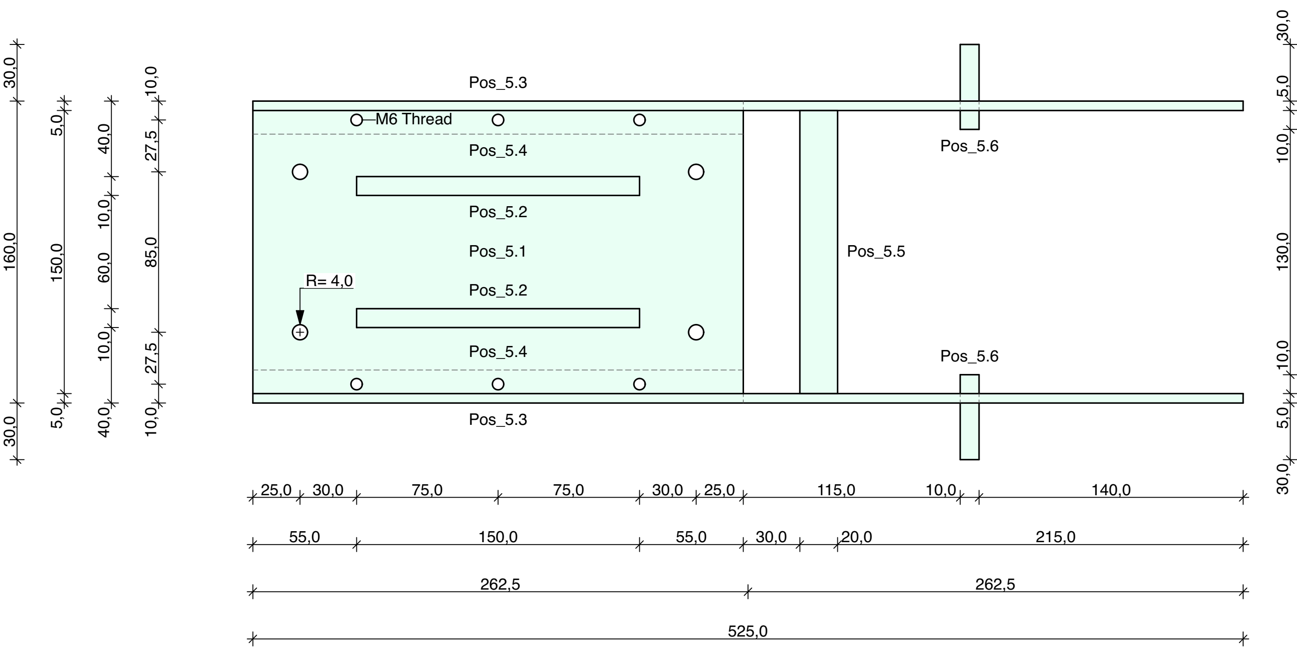
Assembly_Top View
