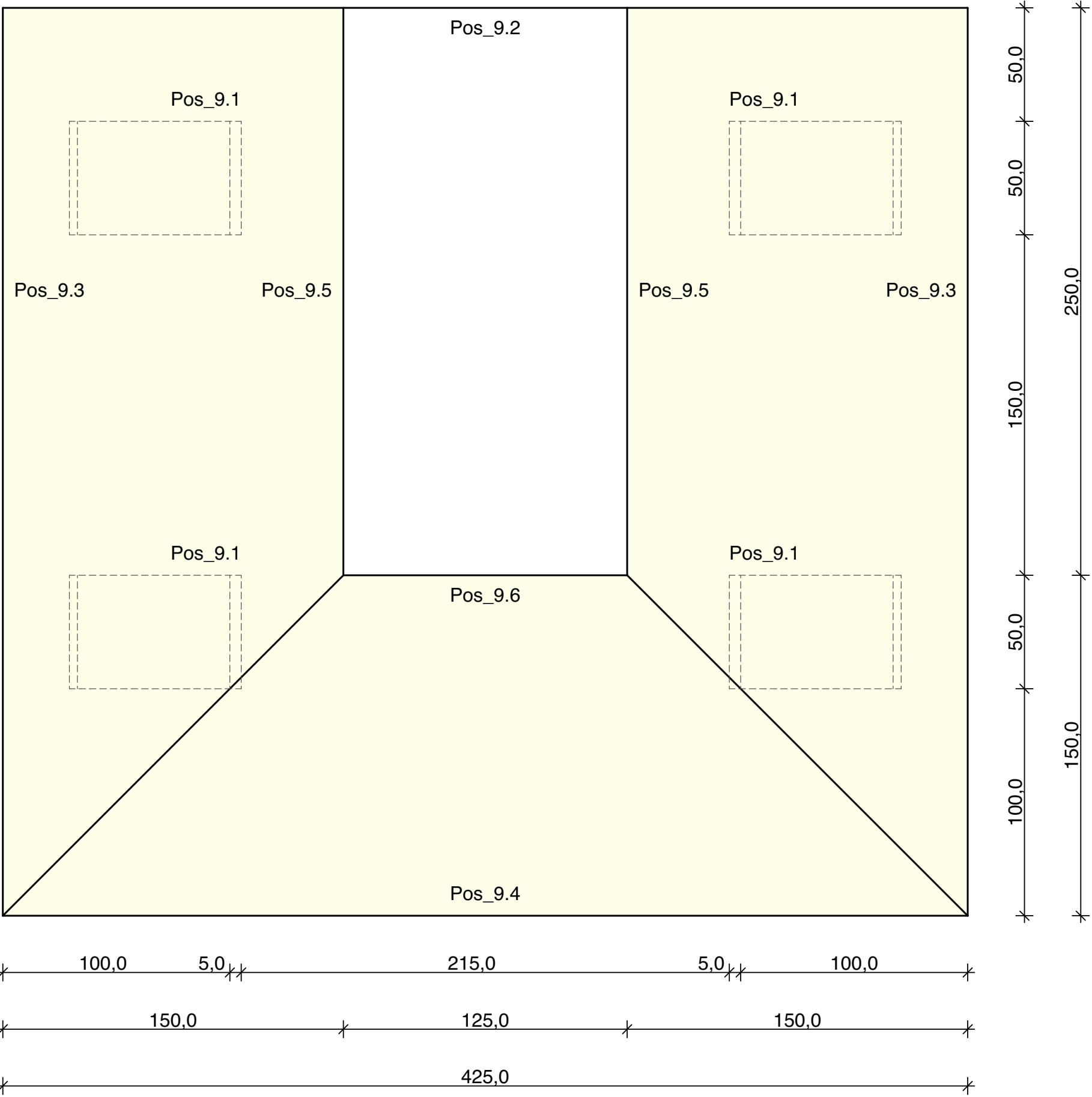
Assembly_Top View
