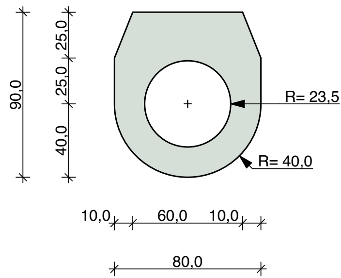
Pos_6.2.4 2 Pieces Sheet Metal 10 mm
