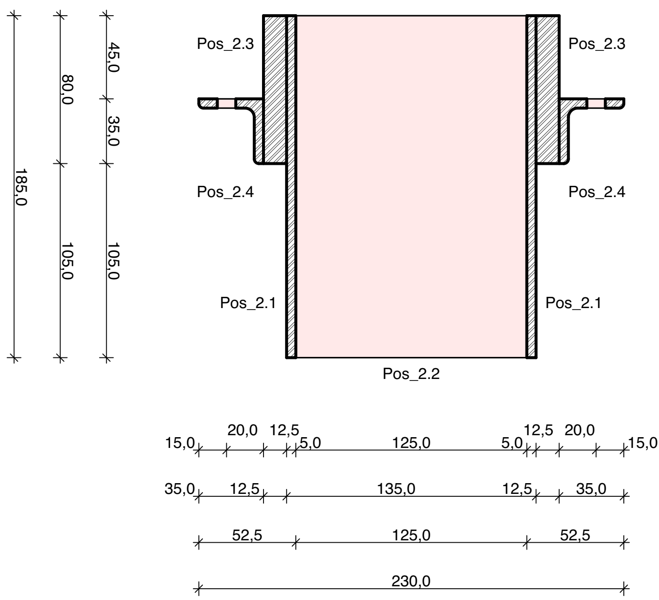
Assembly_Section
