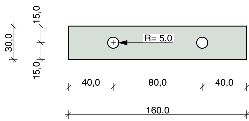
Pos_3.11 1 Piece Hard Plastic 5 mm
