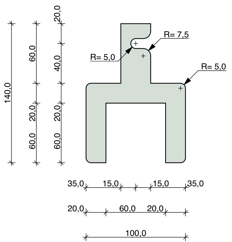
Pos_6.2.3 1 Piece Sheet Metal 10 mm
