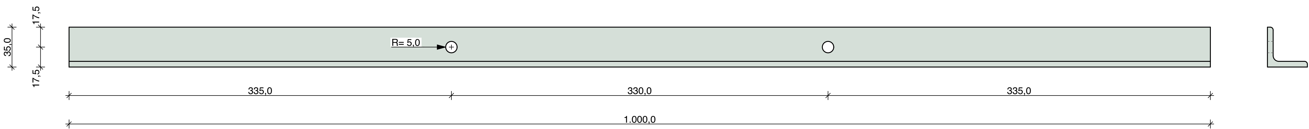
Pos_3.23 2 Pieces L-Section 35 x 35 x 5 mm
