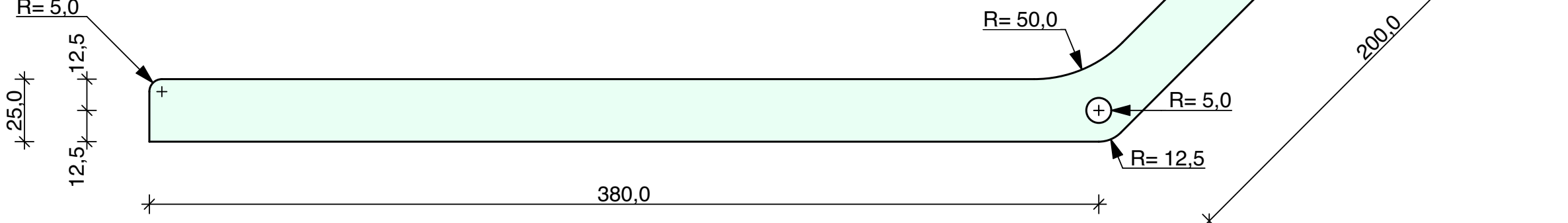
Pos_5.3 2 Pieces Sheet Metal 5 mm
