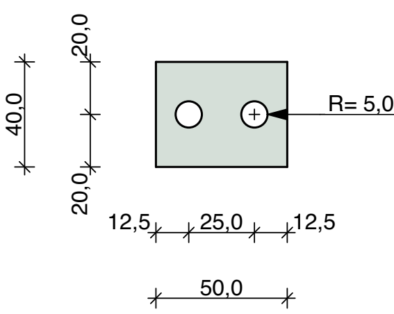
Pos_3.19 4 Pieces Sheet Metal 5 mm
