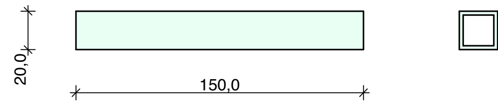
Pos_5.5 1 Piece Square Hollow Section 20 x 20 x 2 mm
