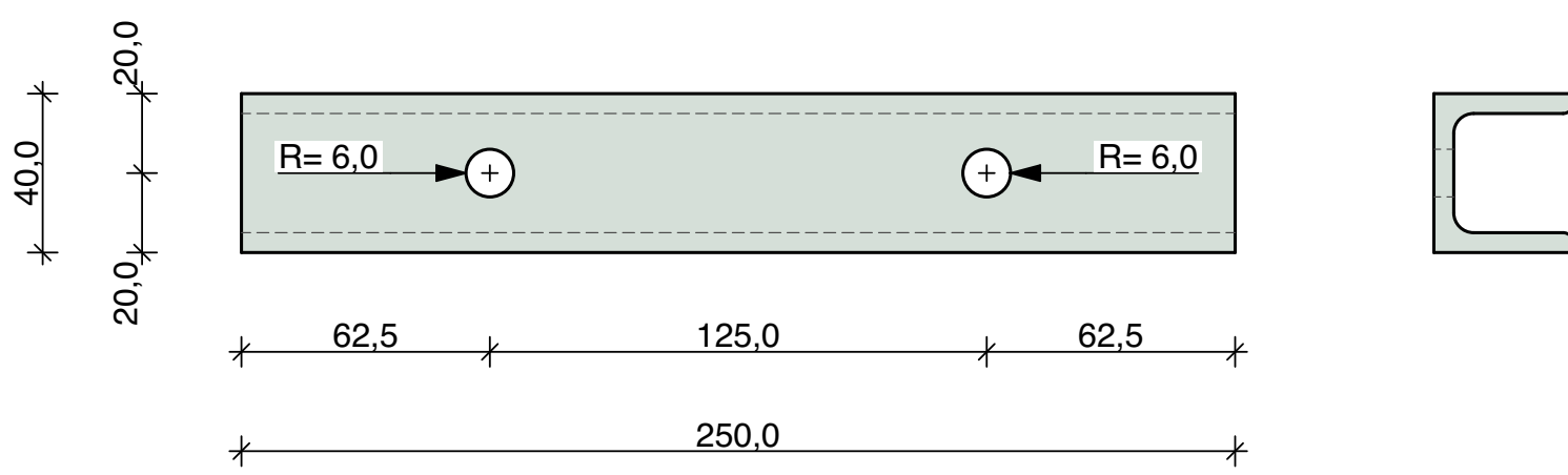
Pos_3.18 1 Piece UPN 40 x 35 mm
