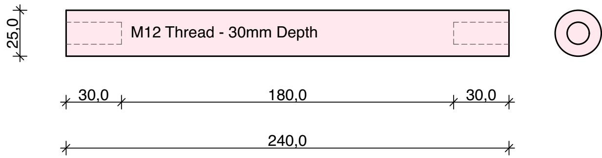
Pos_4.9 1 Piece Shaft 25 mm
