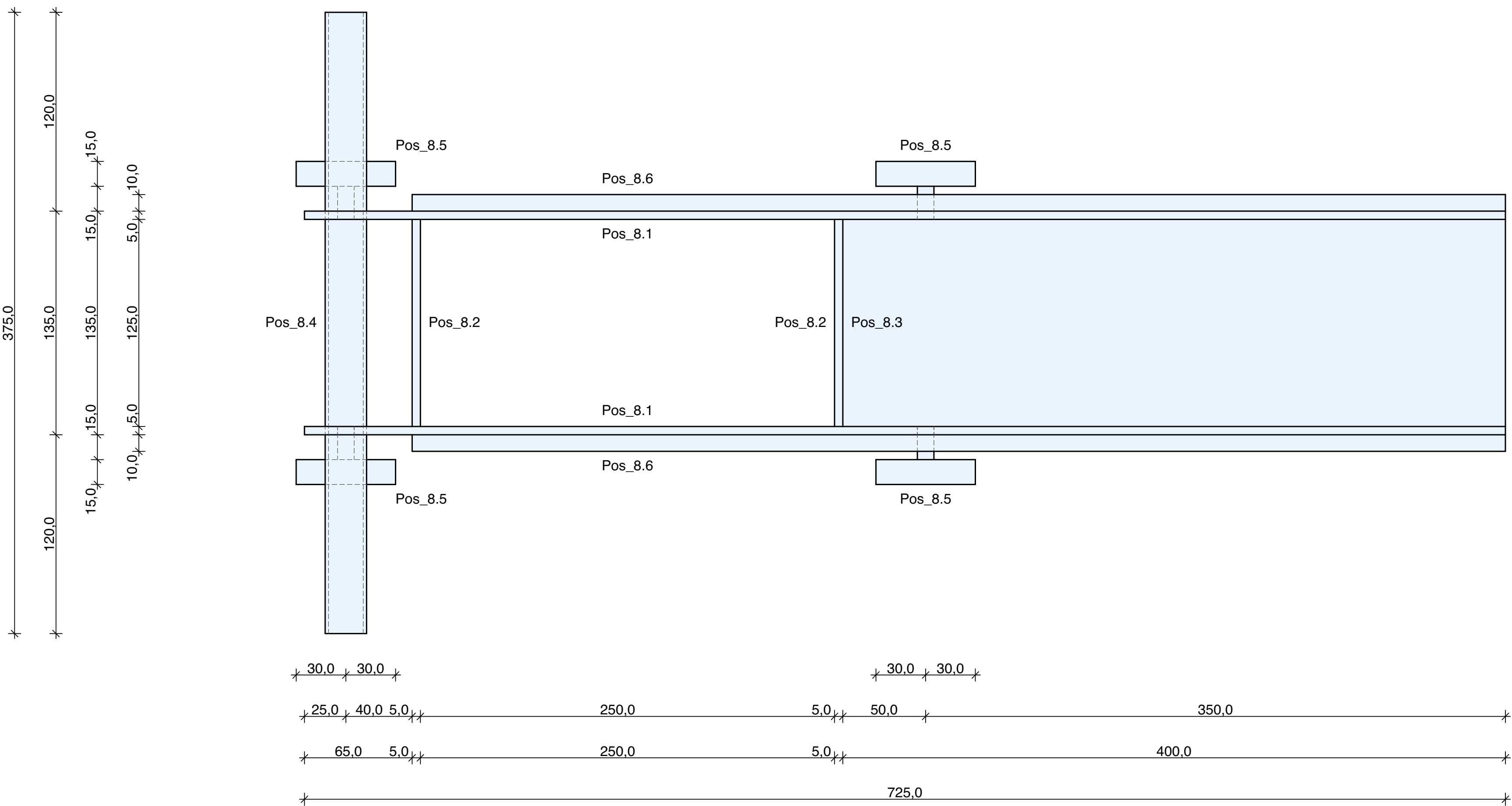
Assembly_Top View
