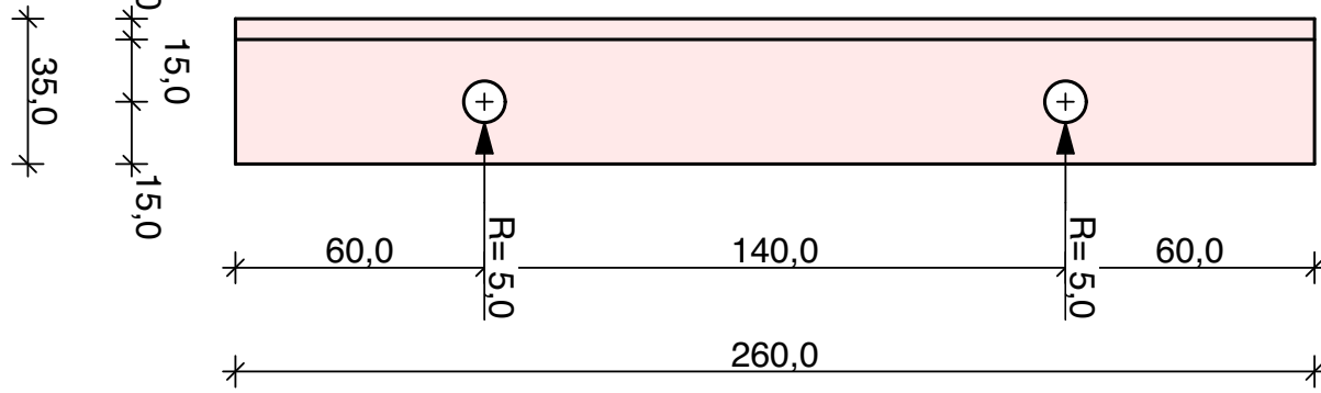
Pos_2.4 2 Pieces L-Section 35 x 35 x 5 mm
