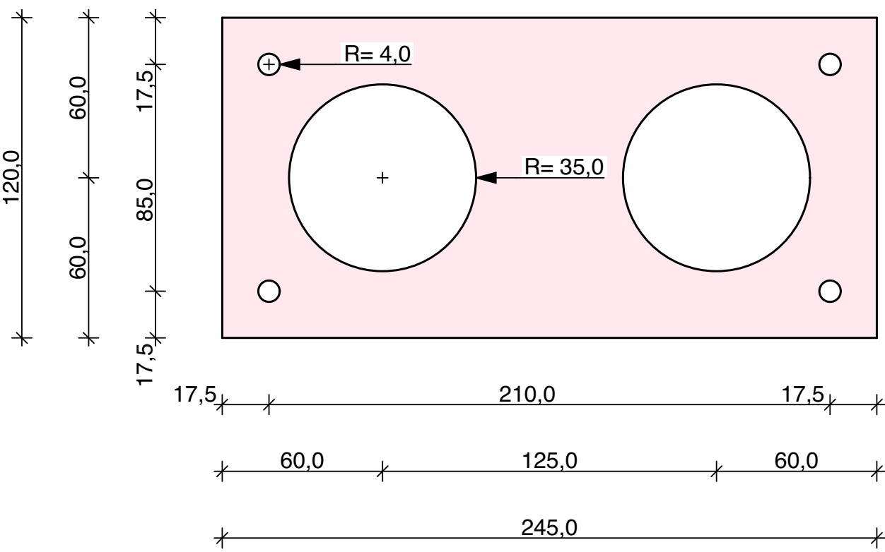
Pos_4.1 1 Piece Sheet Metal 5 mm
