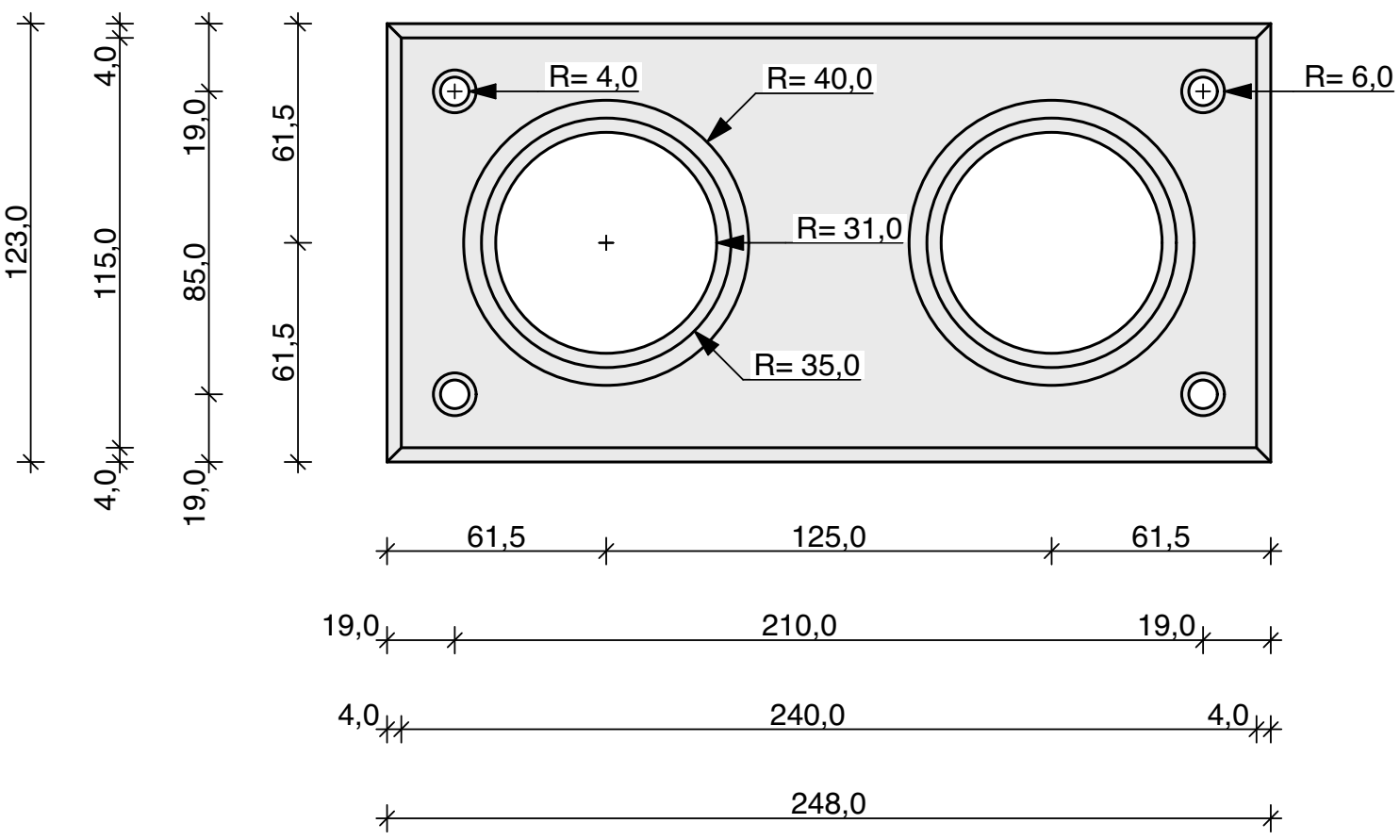
Pos_1.2 1 Piece CNC Aluminum Bottom Piece
