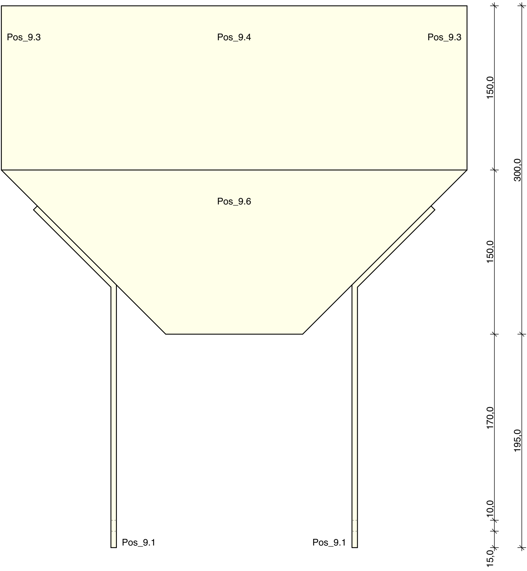
Assembly_Side View
