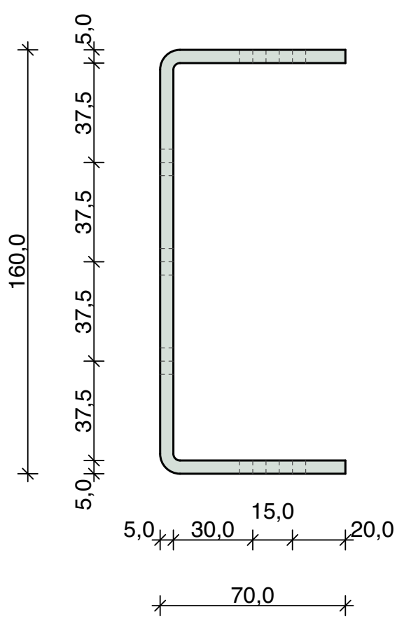
Pos_3.1 1 Piece Sheet Metal 5 mm, bent
