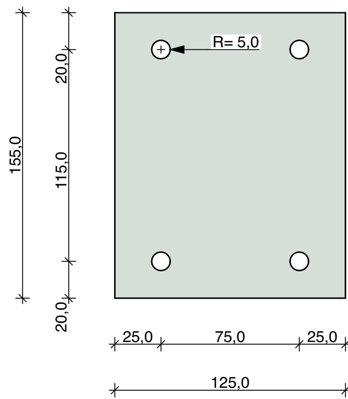
Pos_3.20 2 Pieces Hard Plastic 5 mm
