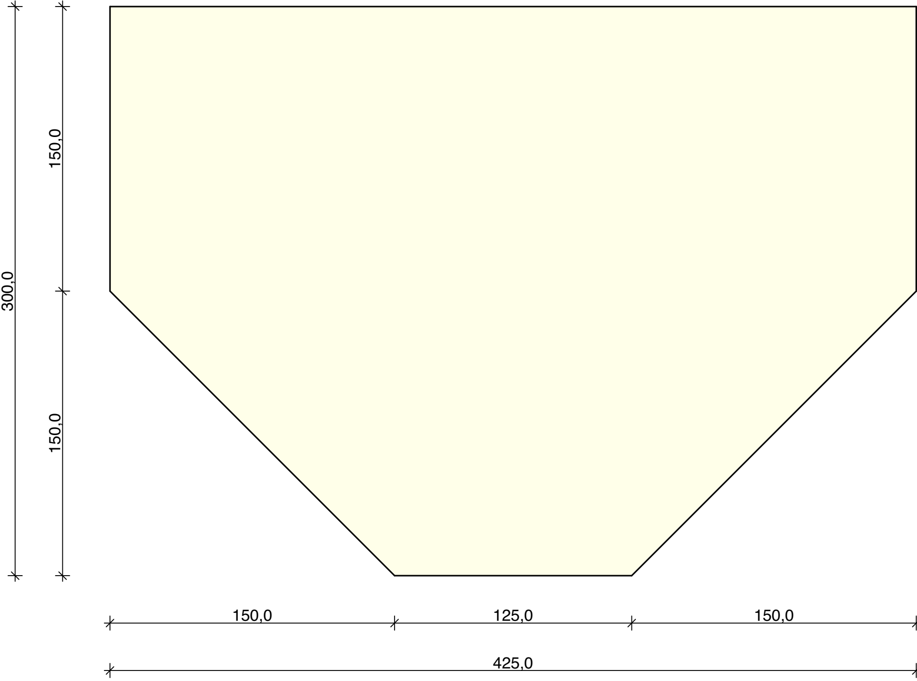
Pos_9.2 1 Piece Sheet Metal 3 mm
