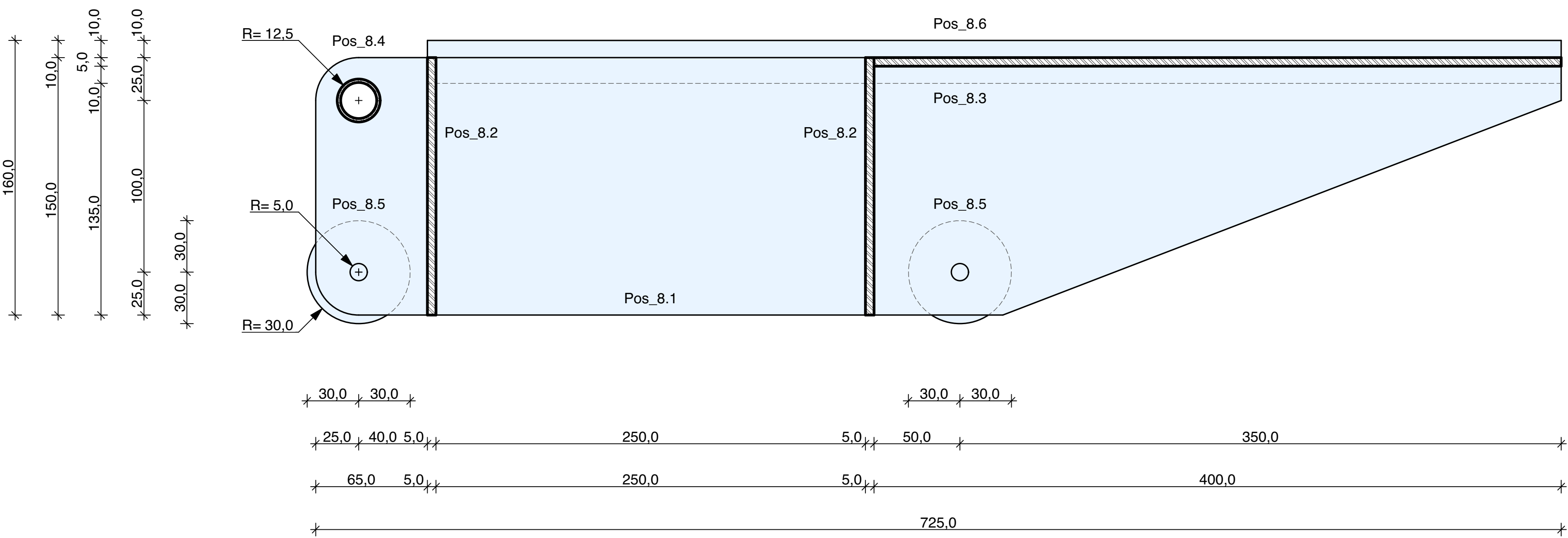
Assembly_Section
