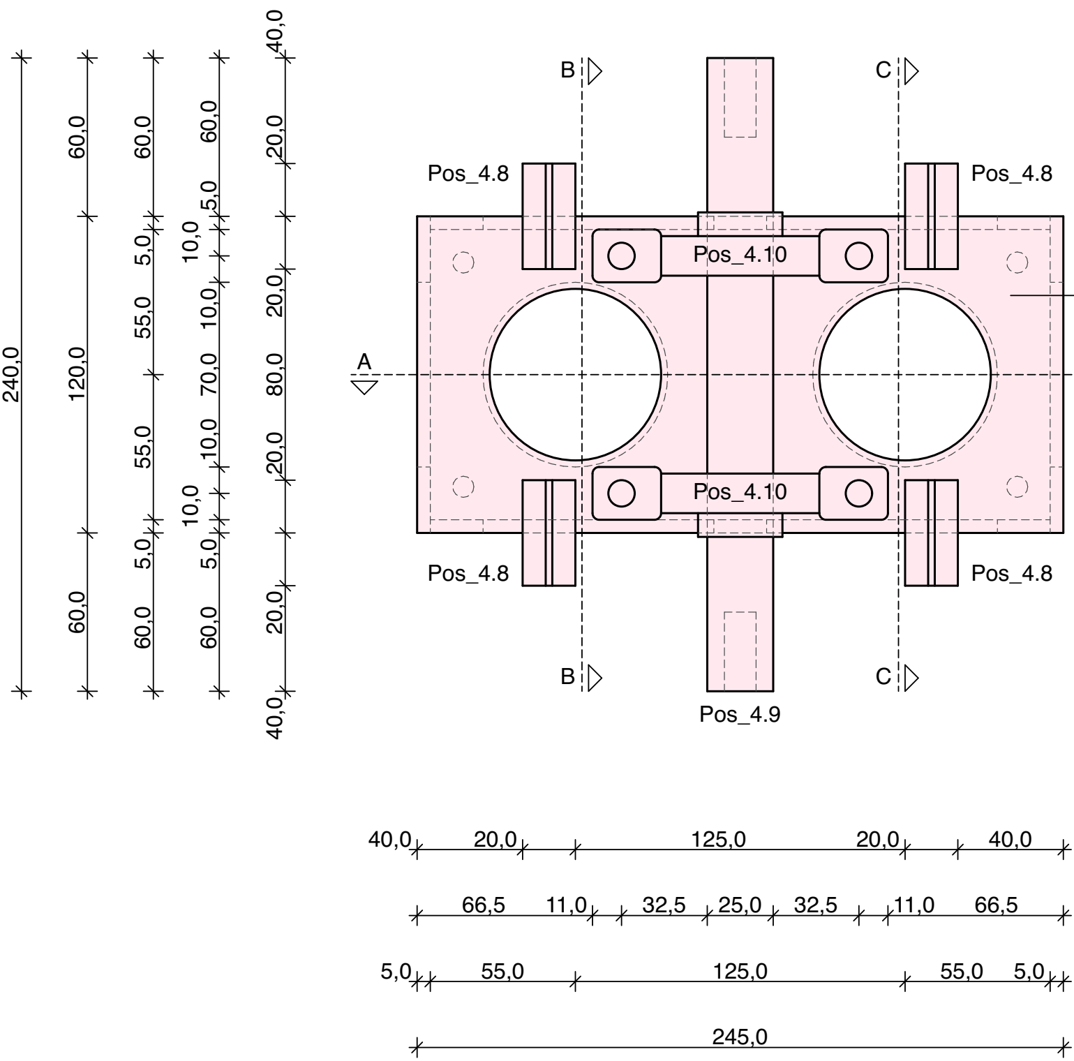
Assembly_Bottom View
