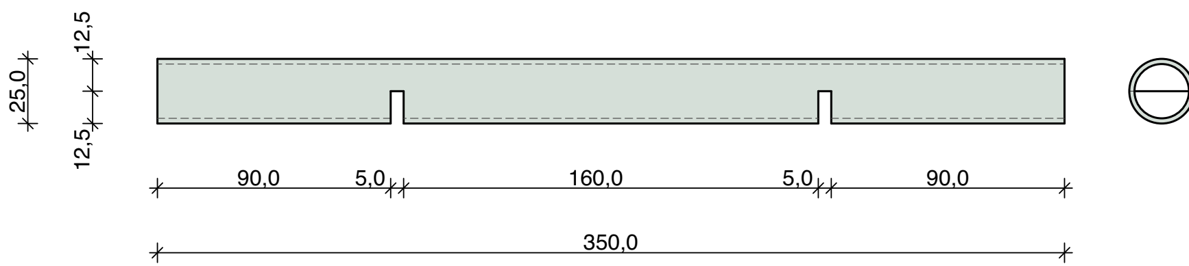
Pos_3.15 1 Piece Circular Hollow Section 25 x 2 mm
