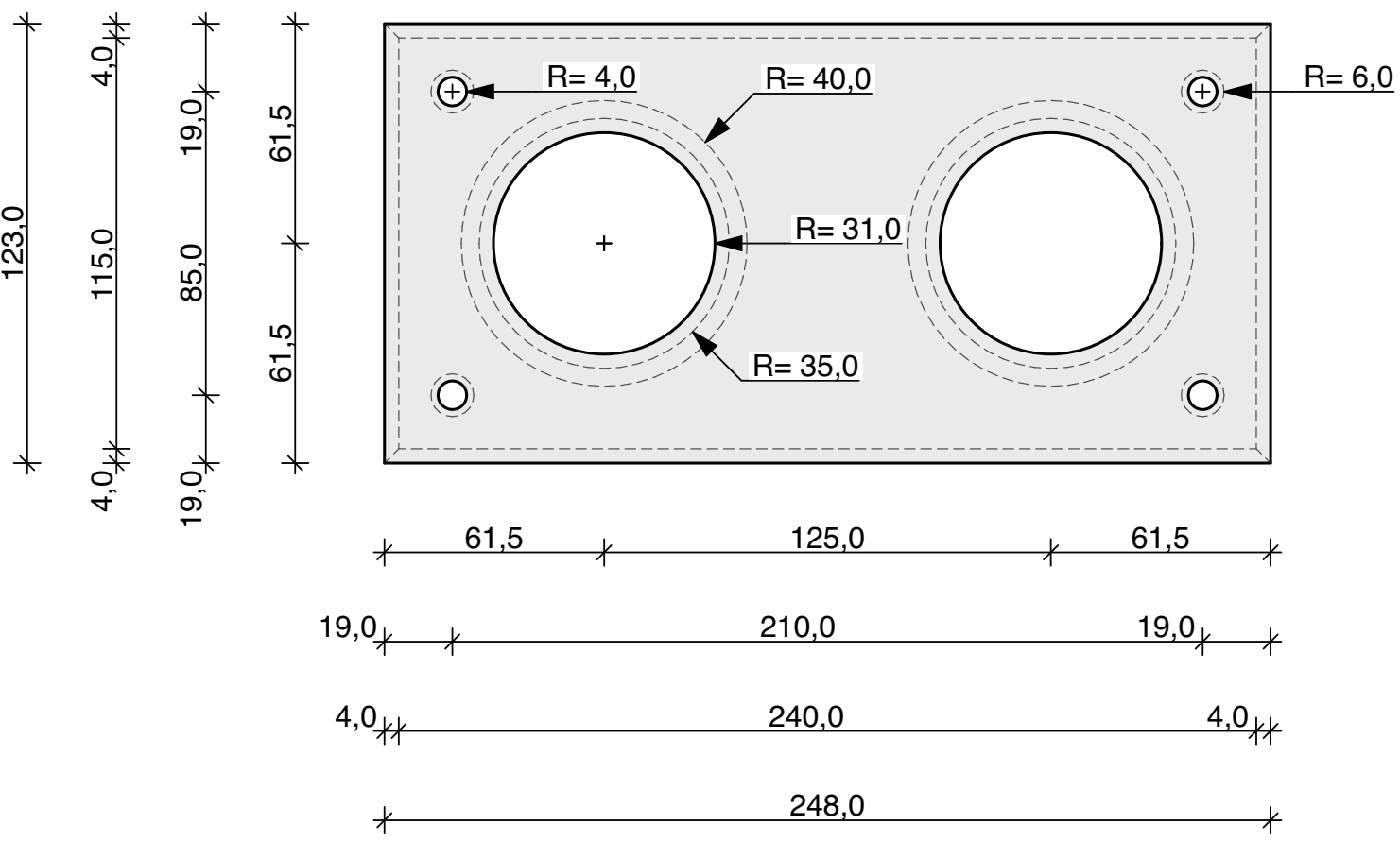
Pos_1.1 1 Piece CNC Aluminum Top Piece
