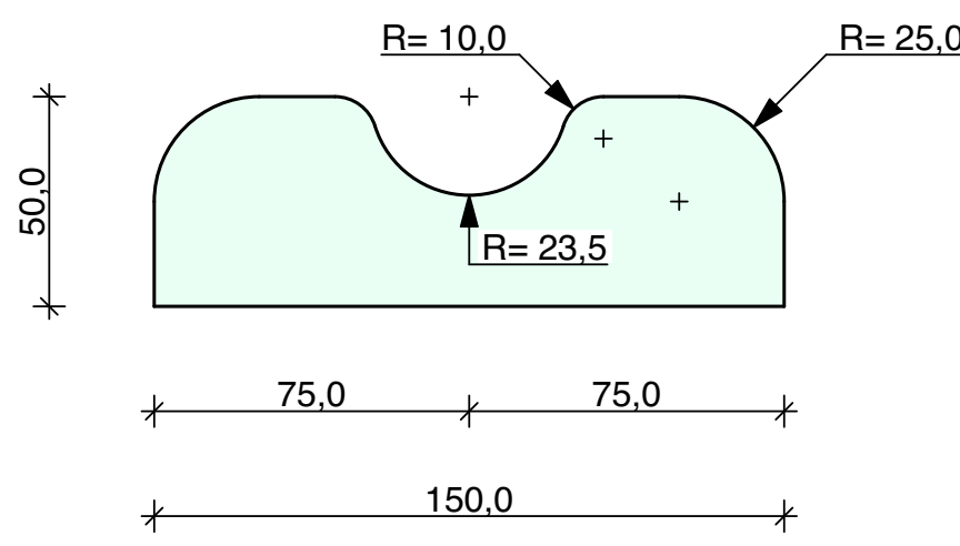
Pos_5.2 2 Pieces Sheet Metal 10 mm
