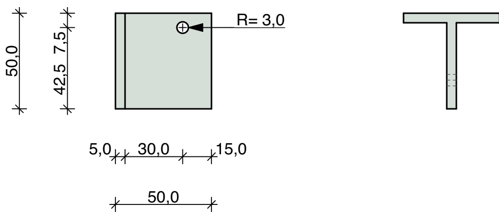
Pos_3.21 1 Piece T-Section 50 x 50 x 5 mm
