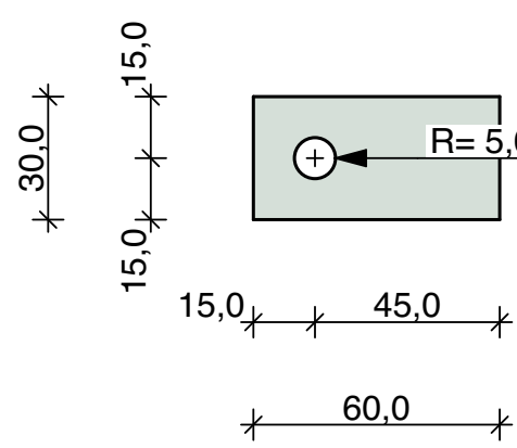
Pos_3.12 2 Pieces Sheet Metal 5 mm
