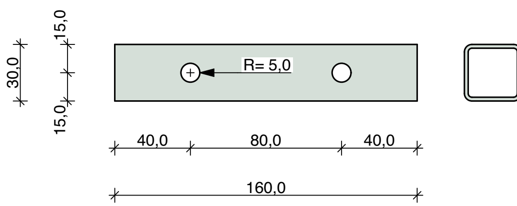
Pos_3.10 1 Piece Square Hollow Section 30 x 30 x 2 mm
