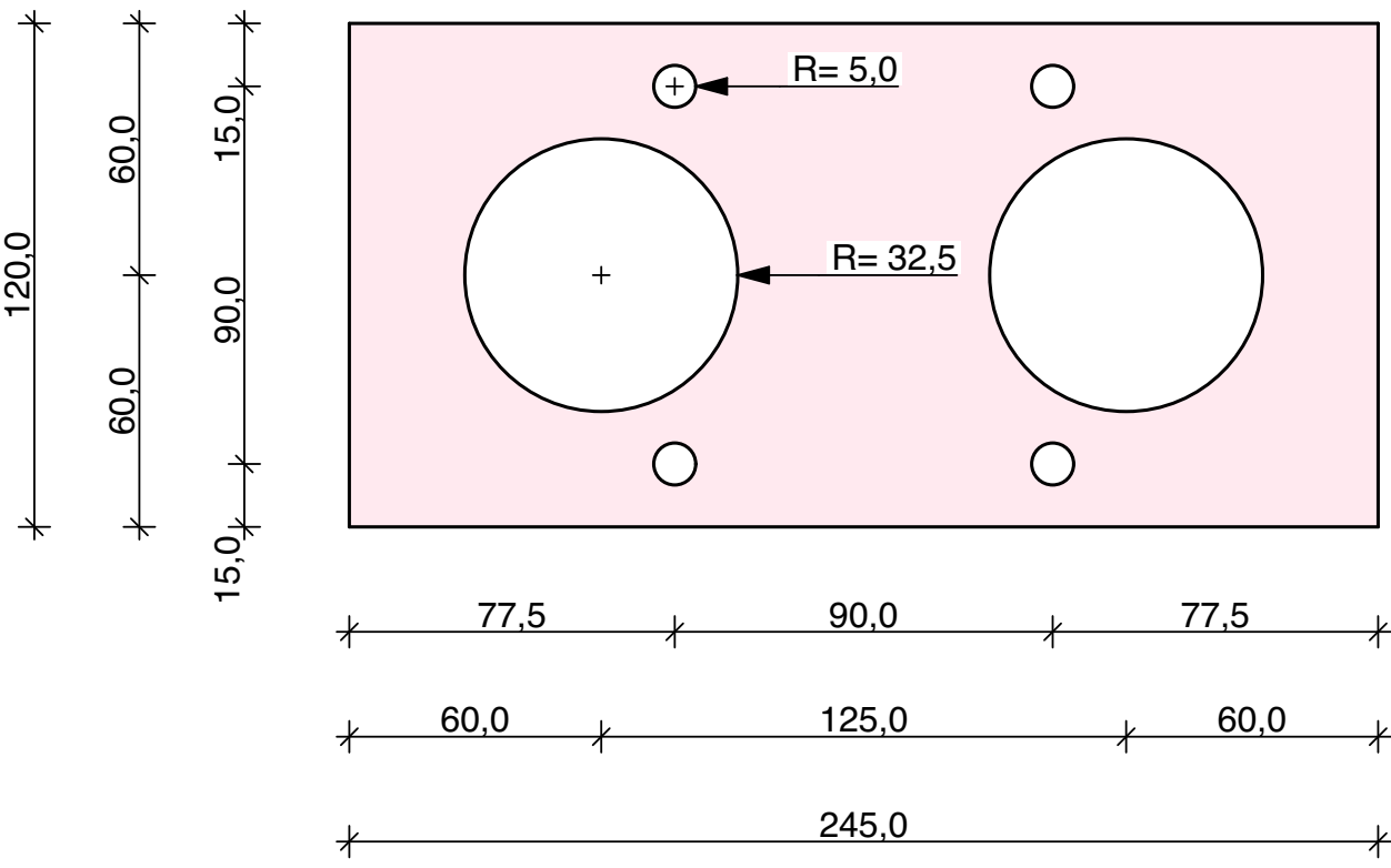
Pos_4.6 1 Piece Sheet Metal 5 mm
