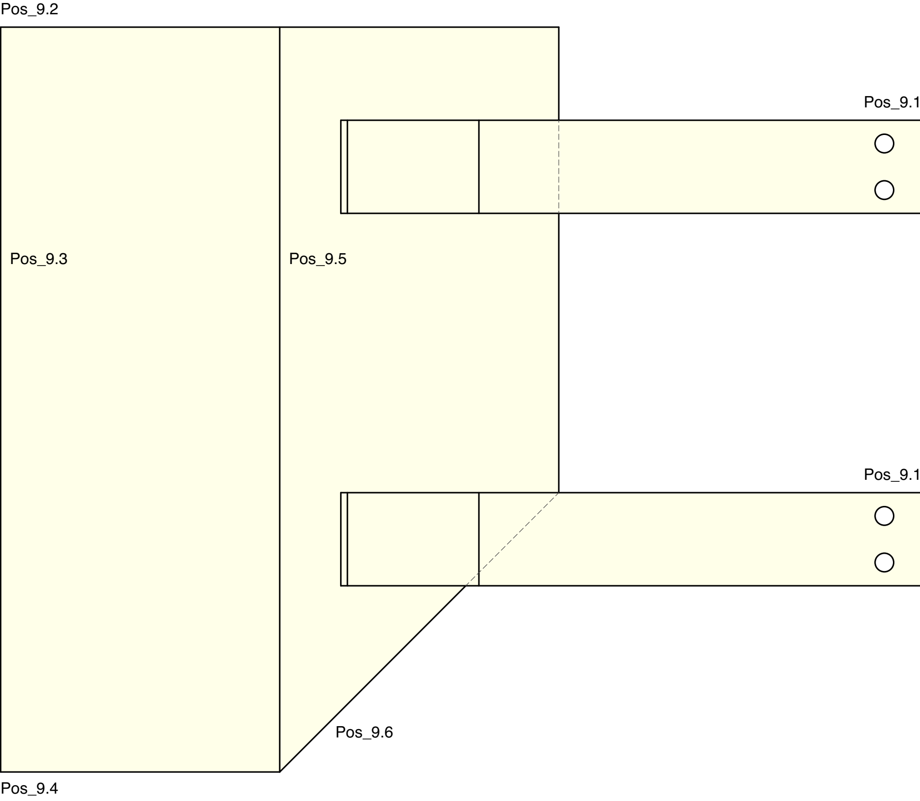
Assembly_Side View
