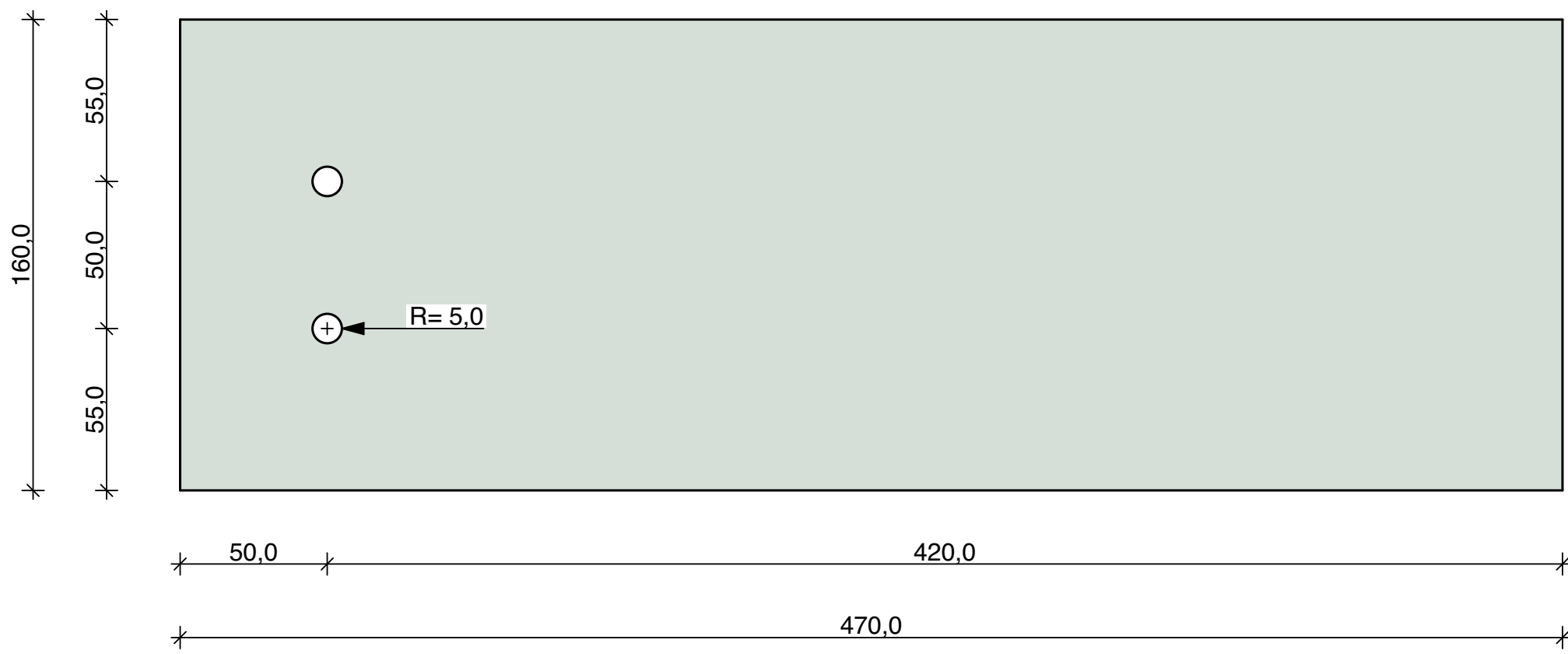
Pos_3.7 1 Piece Sheet Metal 5 mm
