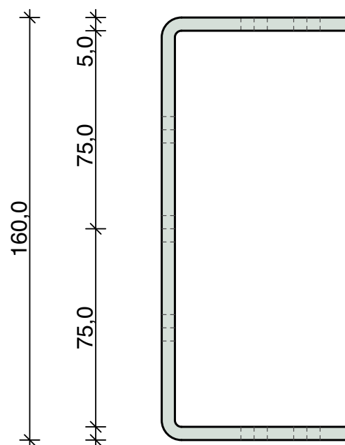
Pos_3.2 1 Piece Sheet Metal 5 mm, bent
