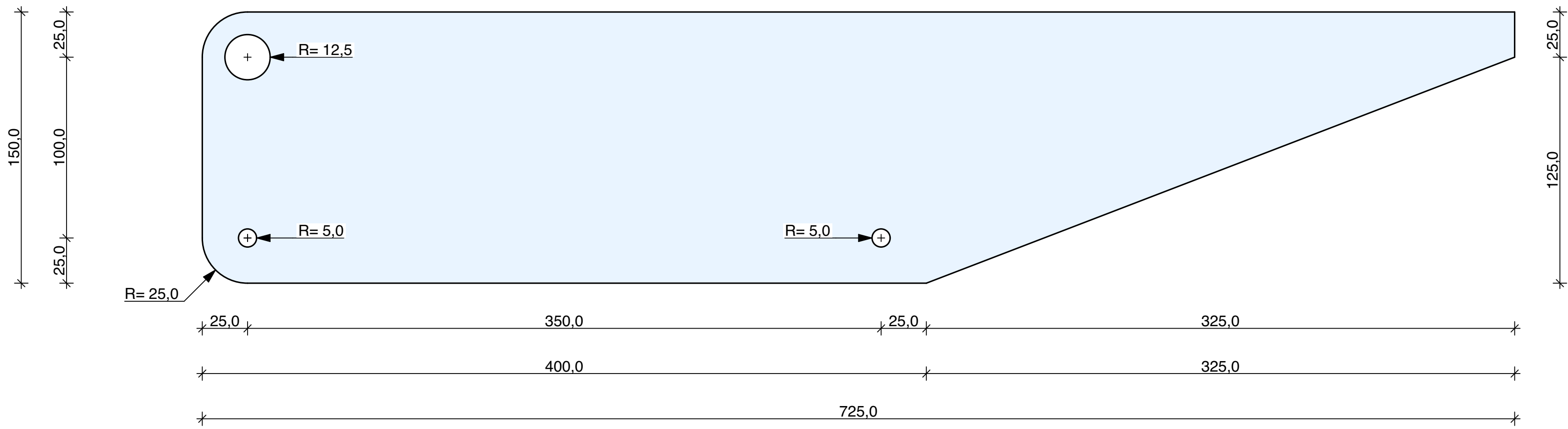
Pos_8.1 2 Pieces
