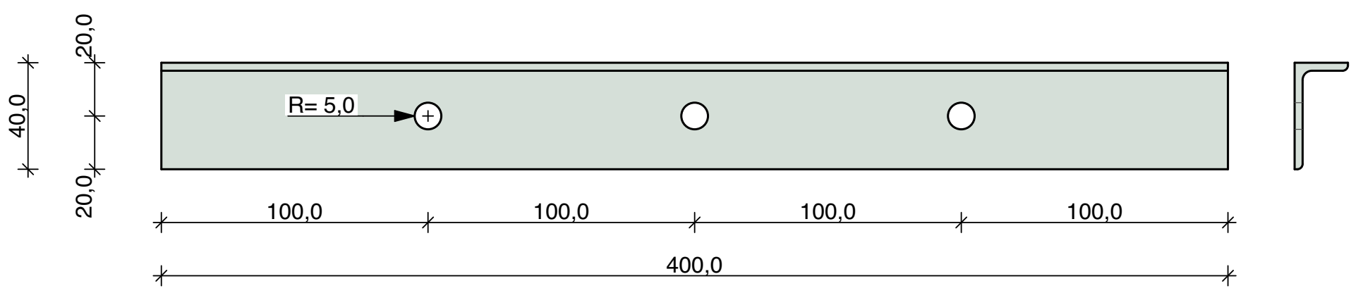
Pos_3.6 2 Pieces L-Section 40 x 20 x 3 mm
